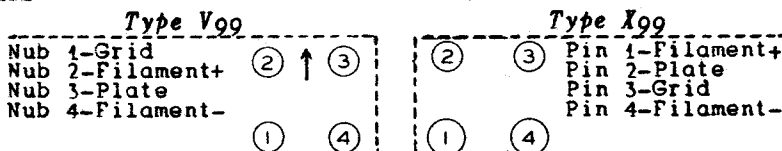
BOTTOM VIEWS
